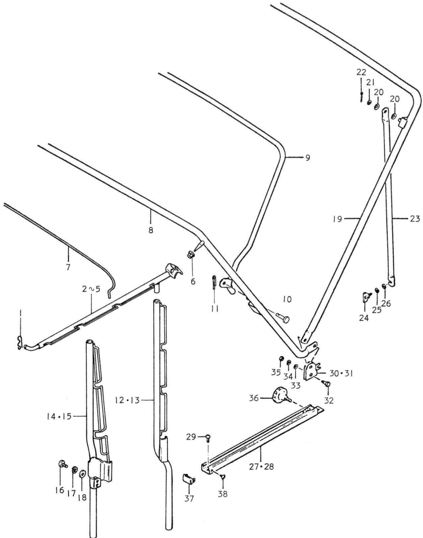
FIG.80 TOP BOW ( low type )
