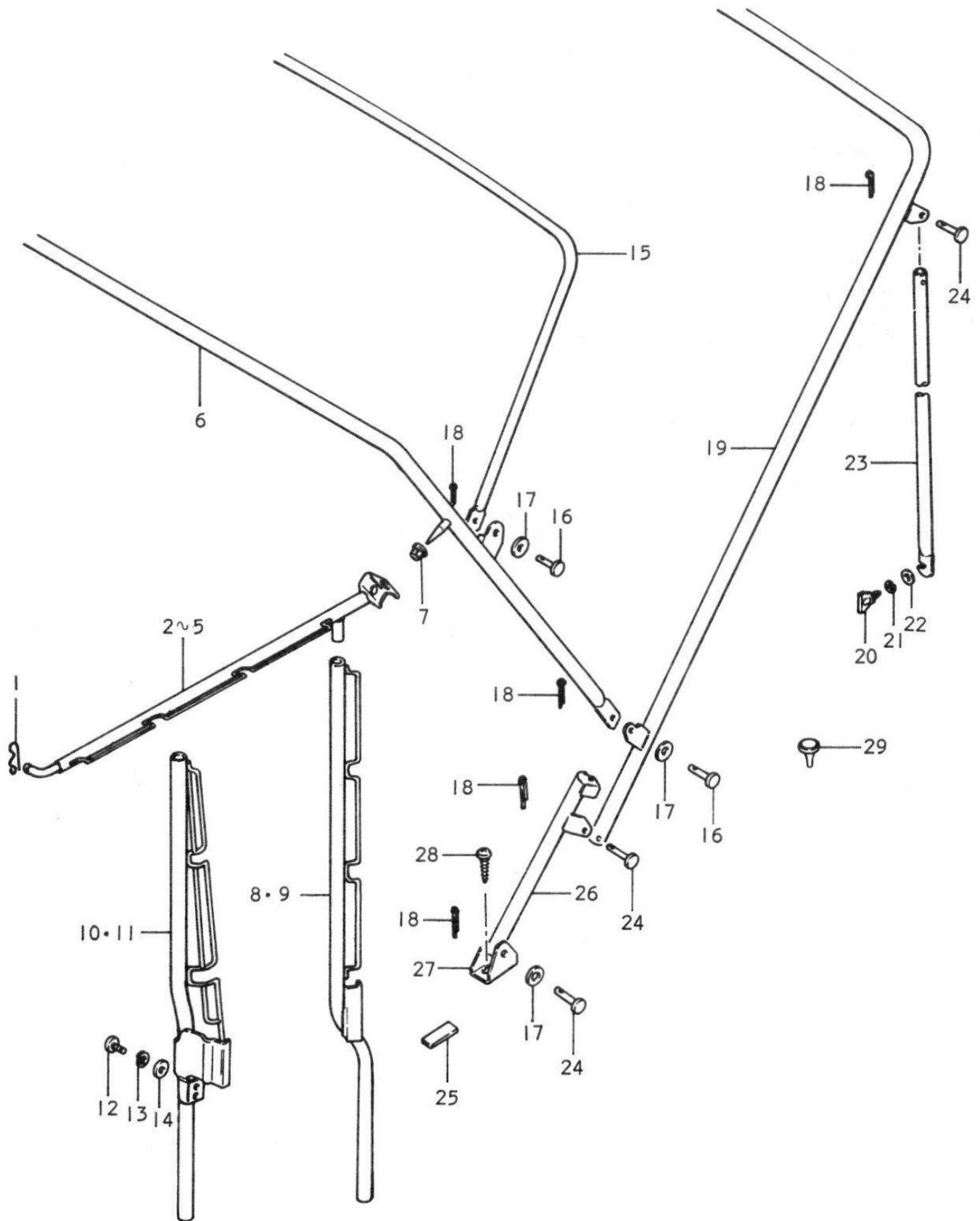
FIG.81 TOP BOW ( high type )
