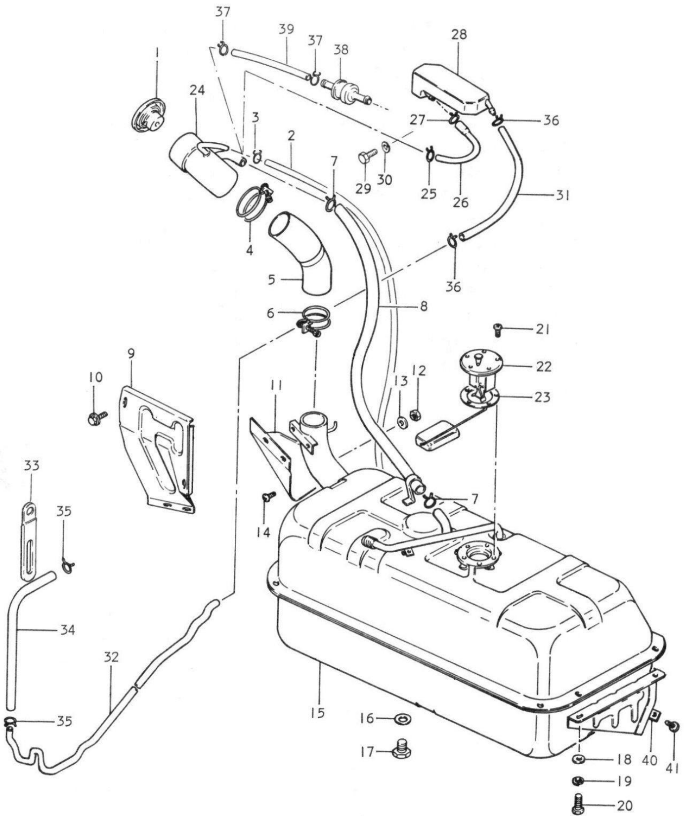
FIG.83 FUEL TANK
