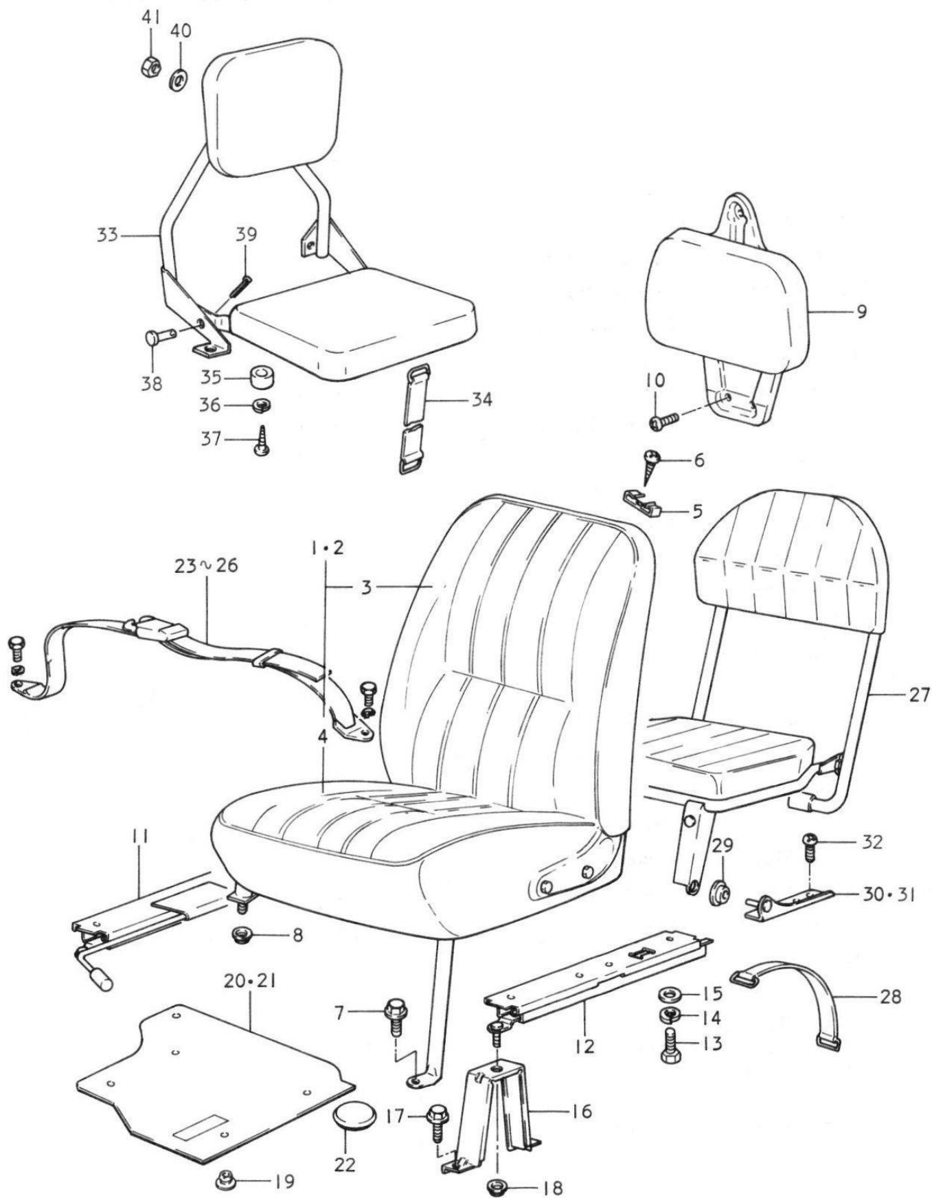
FIG.82 SEAT
