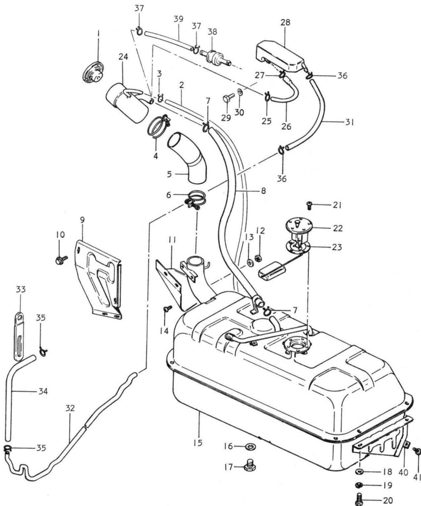
FIG.83 FUEL TANK
