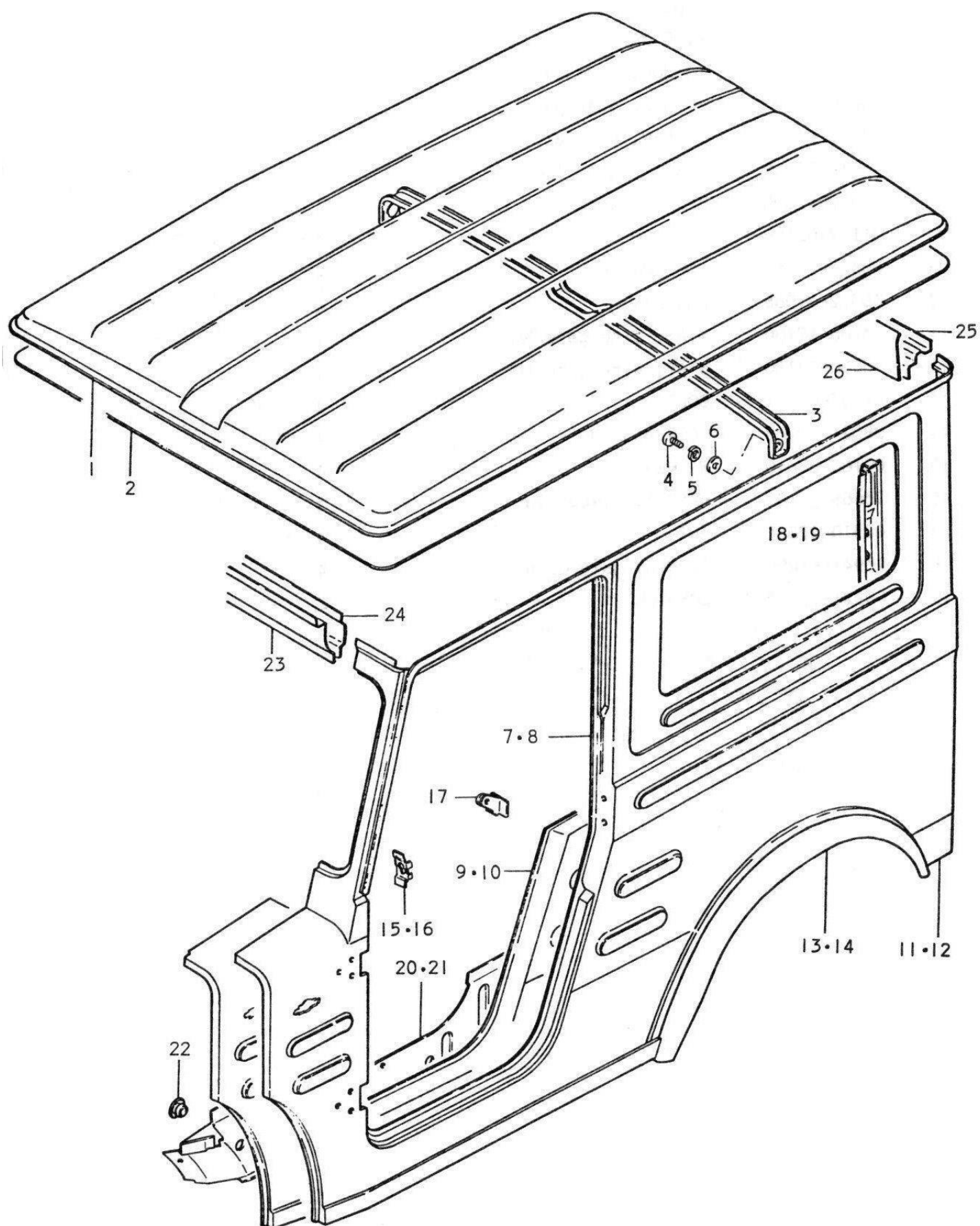
FIG.70 SIDE BODY
