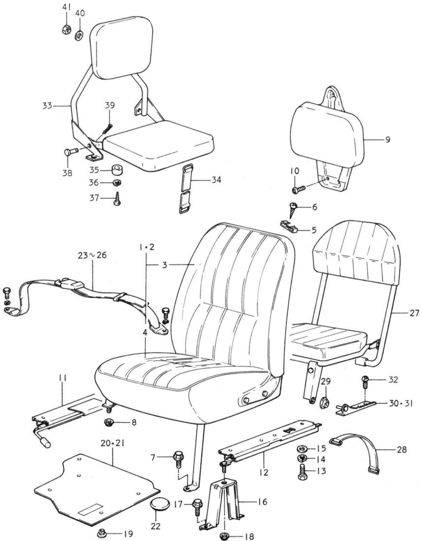
FIG.82 SEAT
